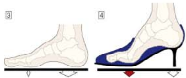
Unhindered by high heels, the strong heel bone can fulfil its function of carrying our bodyweight (Fig. 3).
